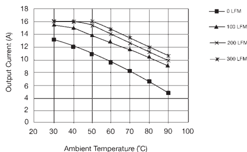
Derating Curve for 5.0 VDC Output
