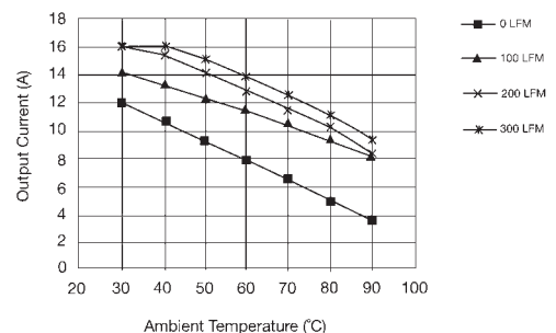
Derating Curve for 5.0 VDC Output
