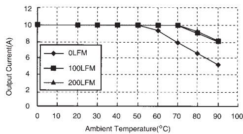
Derating Curve for 3.3 VDC Input
