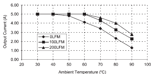
SMT Version Derating Curve for 3.3 VDC Output
