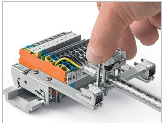
The spring is released by pressing the two actuating elements on the side, firmly securing the shield clamping saddle on the busbar.
