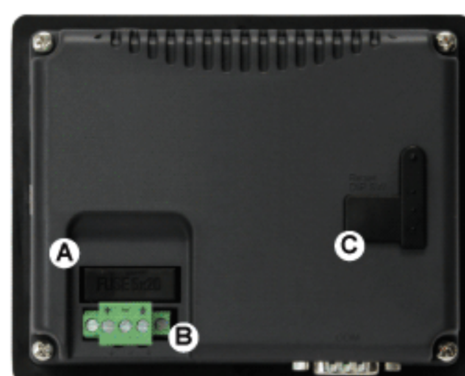
Rear View
