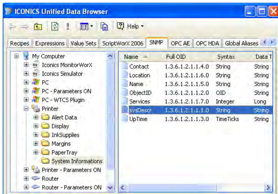
Selecting SNMP Tags from the Unified Data Browser
