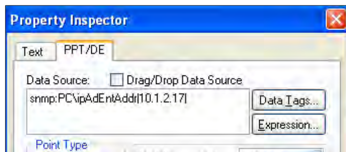
SNMP Tag Syntax Shown in Property Inspector
