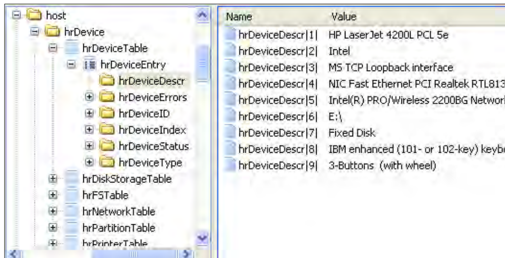
Branch of the Tree in SNMP Explorer With Loaded MIB Items Tree
