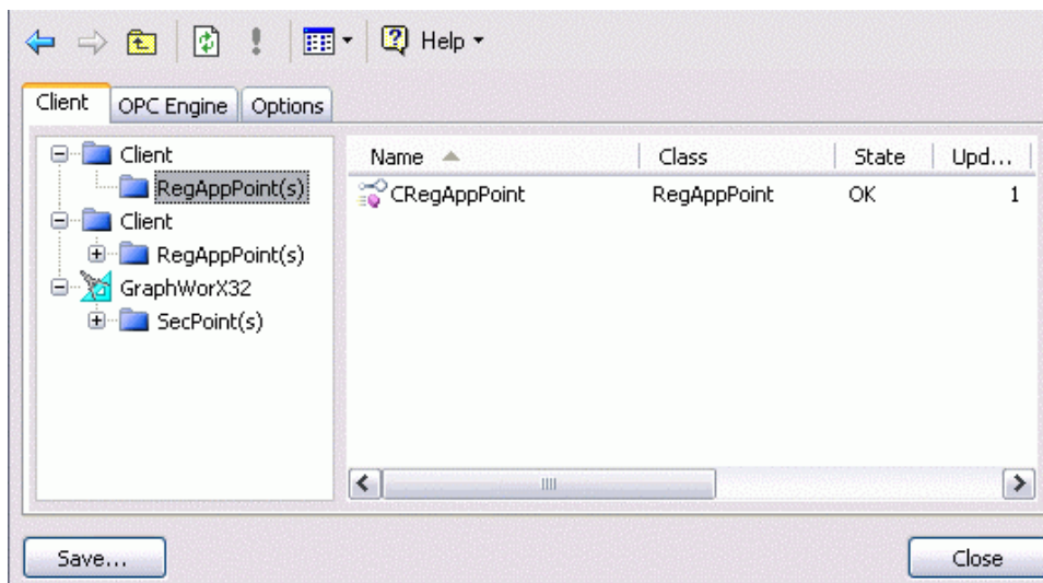
GenStatistics Runtime Viewer
