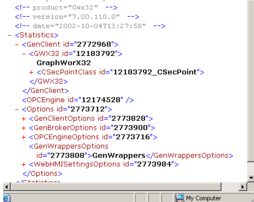
Viewing the Exported XML Statistics File
