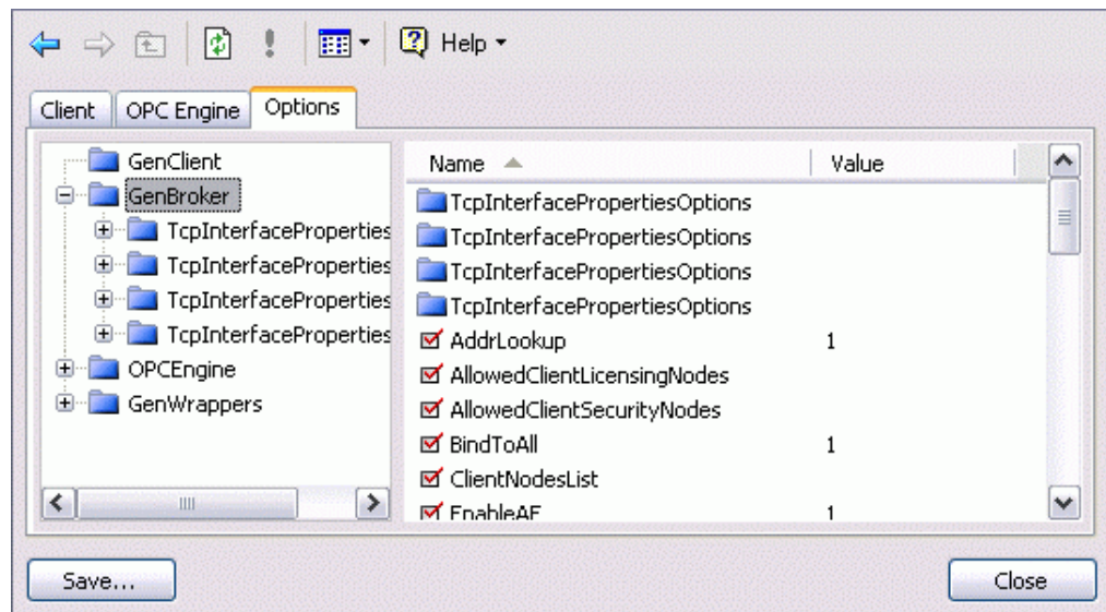
GenStatistics Runtime Viewer: Options Tab
