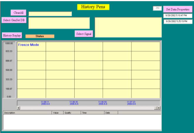
Figure 1 - HistoryPen.t32 Runtime
