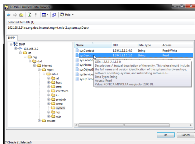
Figure 3 - Browse for SNMP Tags
