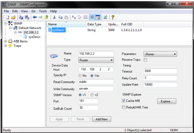
Figure 4 - SNMP Tag Added to the Configuration
