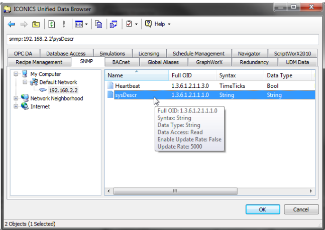
Figure 5 - Browsing for SNMP Tags from Unified Data Browser
