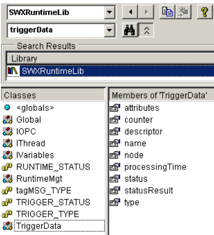
Figure 1 - TriggerData Members
