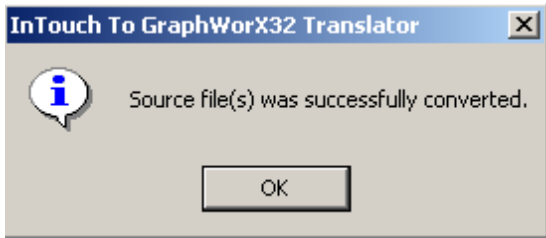
Figure 8 - Confirmation Dialog
