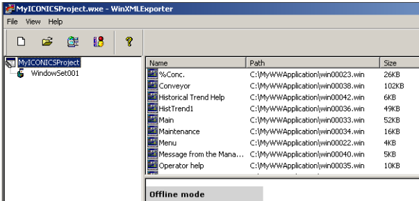
Figure 5 - WinXML Exporter
