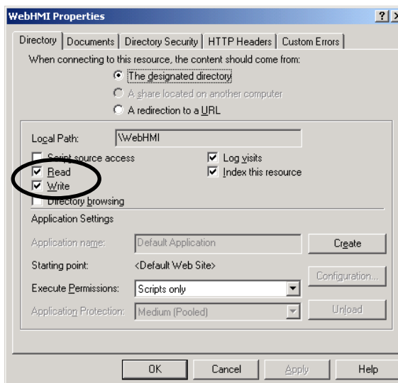
Figure 3 - WebHMI Properties
