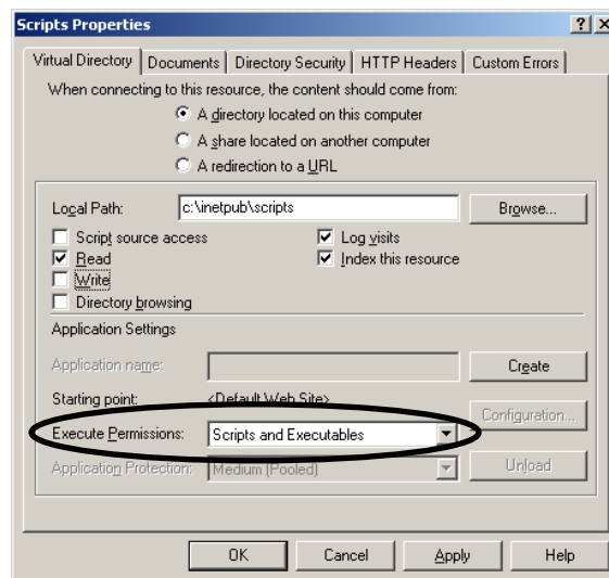
Figure 2 - Scripts Properties
