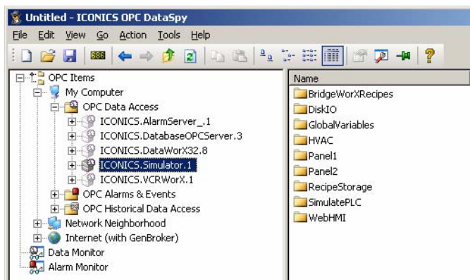
Figure 1 - OPC DataSpy
