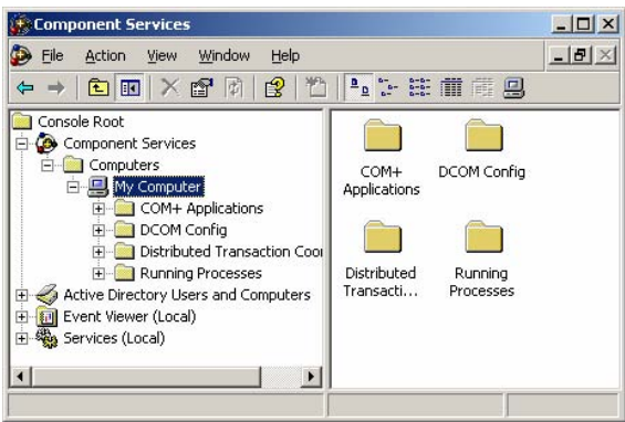
Figure 1 - Component Services
