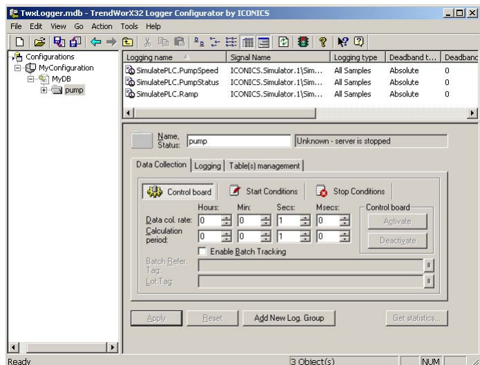
Fig.2 Complete Configuration with OPC Tags
