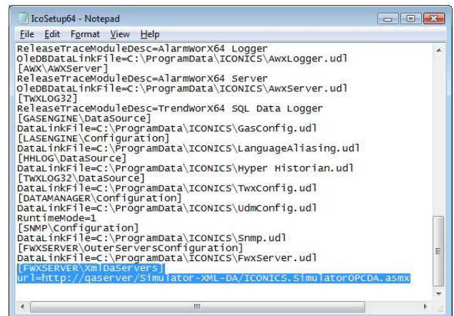
Figure 5 - Setting up OPC XML-DA Servers
