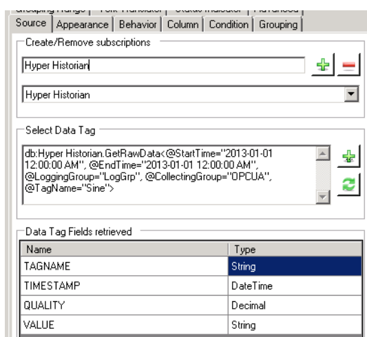
Figure 4 - GridWorX64 Viewer Source tab
