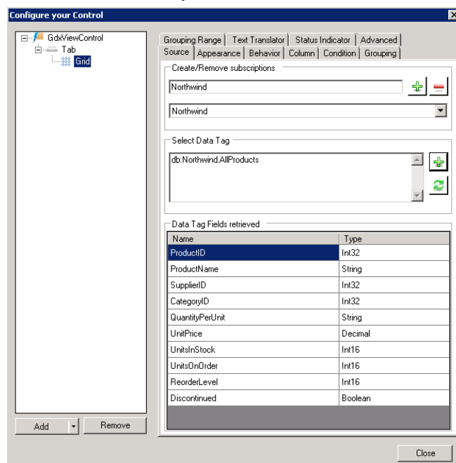
Figure 1 - GridWorX64 Viewer Source configuration
