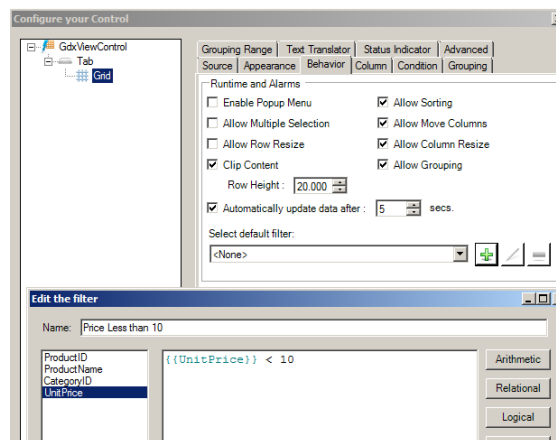
Figure 2 - Setting a filter for a GridWorX64 Viewer
