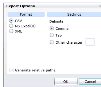
Figure 2 – Export Options
