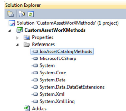
Figure 1 - Referenced IcoAssetsCatalogMethods.dll
