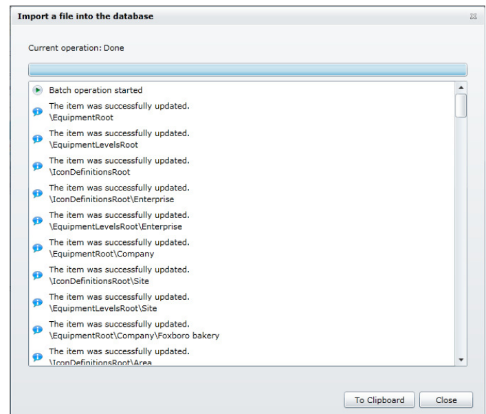
Figure 3 - Import log
