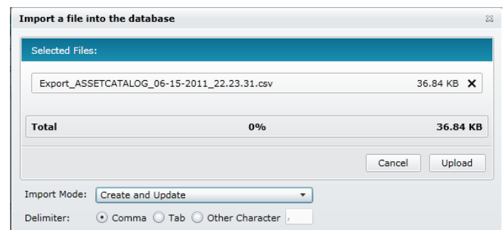
Figure 4 – Import dialog
