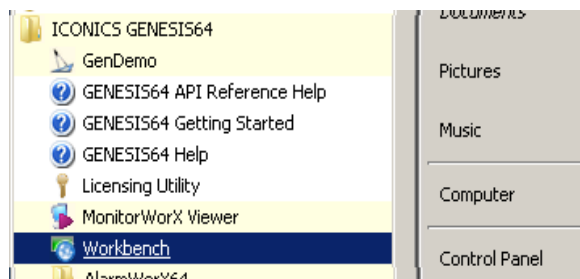
Figure 1 – Workbench64
