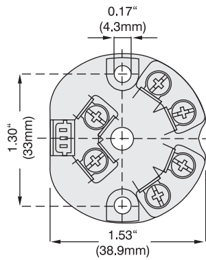
SCTP20-01 Input/Output Not Electrically Isolated
