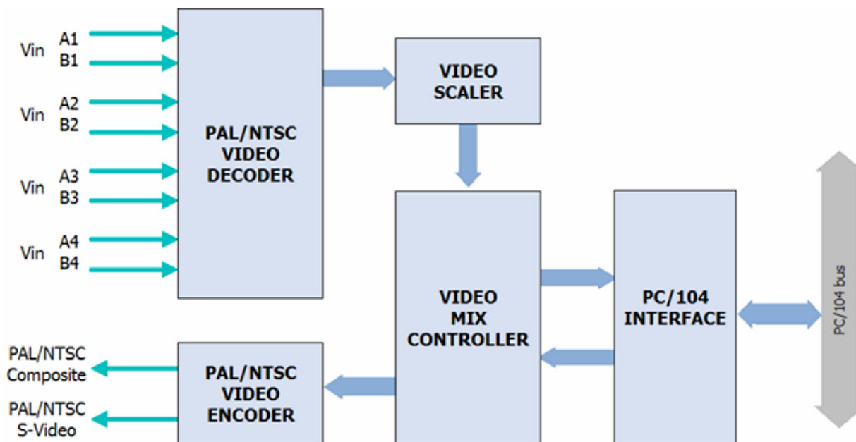
VMIX104 Block Diagram
