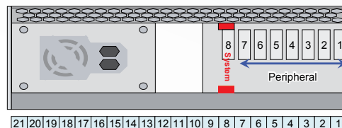
cPCIS-2630R Inside Rear View
