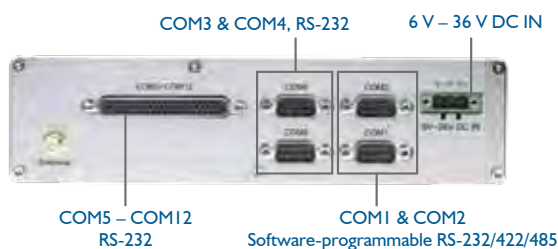
MXE-I212/232 Back Panel
