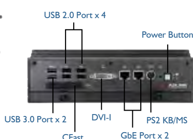
MXE-5300 Front Panel
