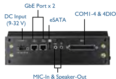
MXE-5300 Back Panel
