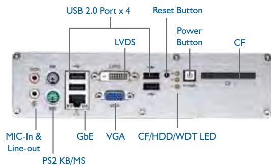
MXE-I200 Series Front Panel
