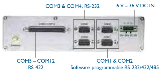
MXE-I212/422 Back Panel
