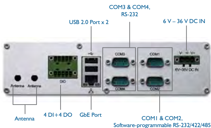
MXE-I300 Series Back Panel
