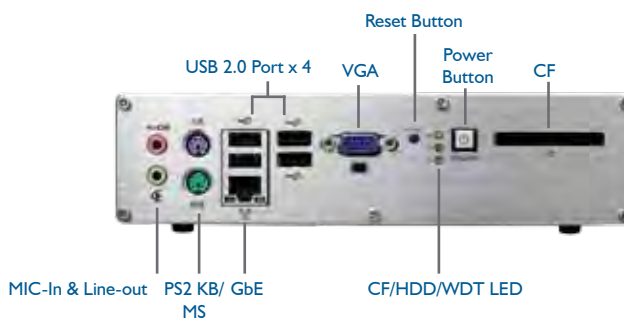
MXE-1000 Series Front Panel
