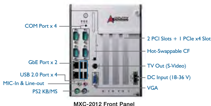
MXC-2012 Front Panel
