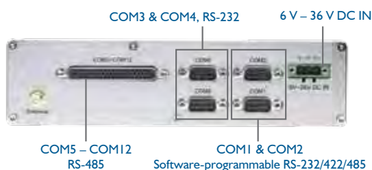
MXE-I212/485 Back Panel
