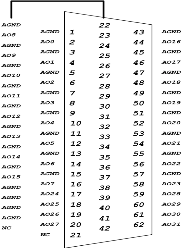
Figure 3.2: I/O Connector Pin Assignments for the PCI-1724U
